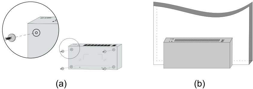
Figure 2-2 Magnet Installation
