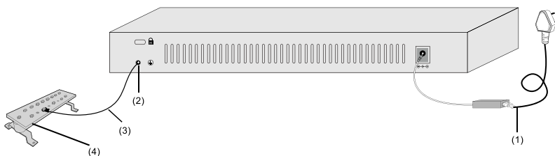
Figure 2-4 Install with grounding bar
