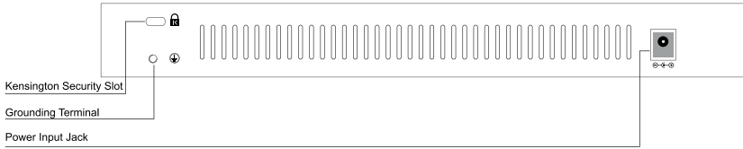
Figure 1-2 Back Panel
