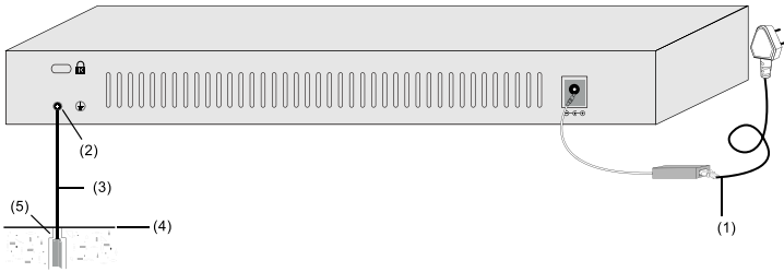
Figure 2-5 Install with a ground conductor buried
